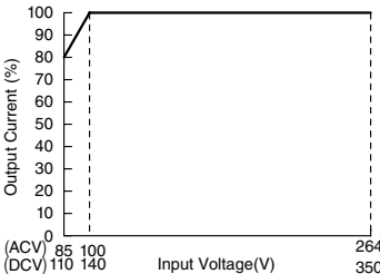
Output Current vs. Input Voltage (Derating Curves) PS9Z-J24 (Ta=25°C)
